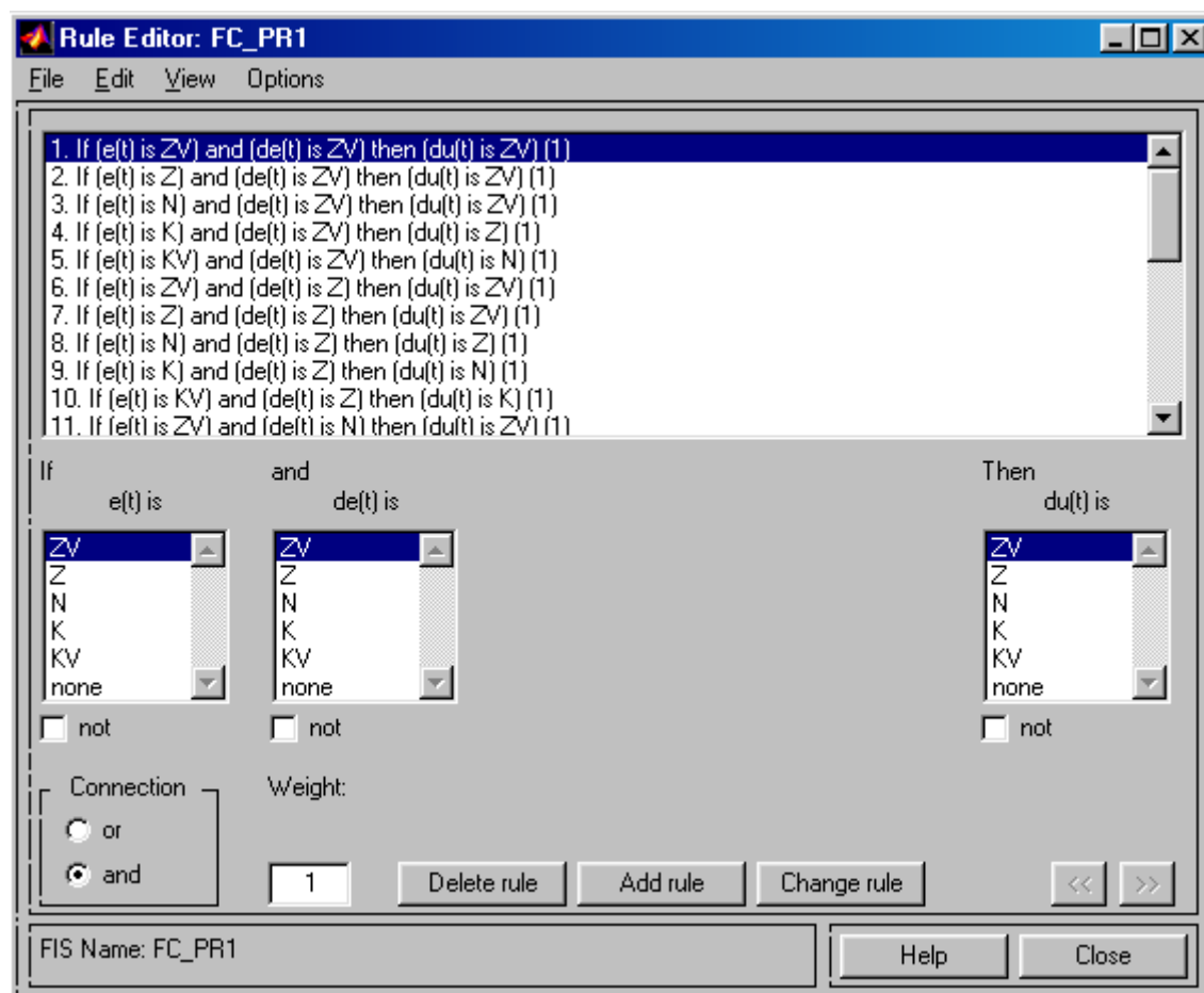
Obr.23. Rules Editor
