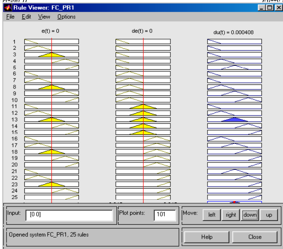
Obr.24 Rule Viewer
