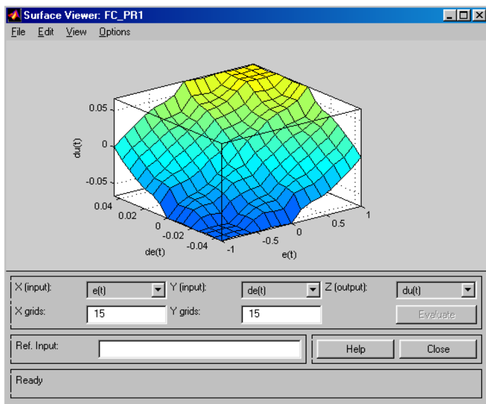
Obr.25 Surface Viewer
