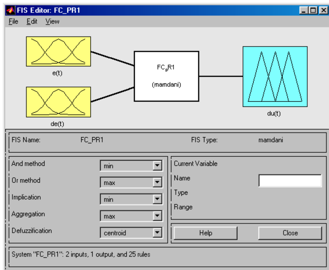
Obr.20 FIS Editor
